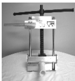
Place tool centrally on the pipe and at 90 0 to the pipe
